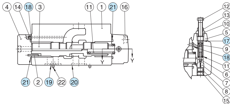
Section Y-Y
